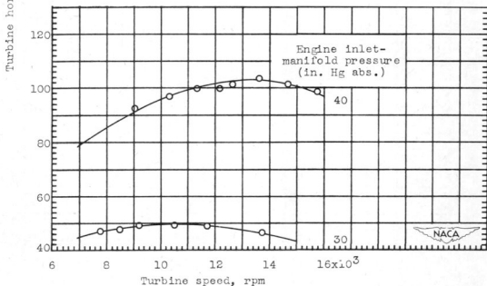
(b) Effect of engine inlet-manifold pressure. Engine speed, 2000 rpm; fuel-air ratio, 0.085; turbine-exhaust pressure, 21 to 22 inches mercury absolute.
