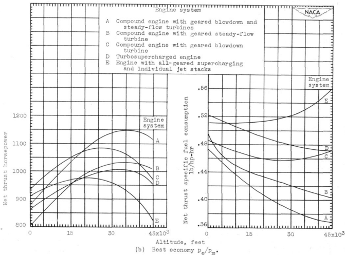
Figure 8. - Concluded. Variation of net thrust horsepower and specific fuel consumption with altitude for five engine systems. Engine speed, 2600 rpm; engine inlet-manifold pressure, 40 inches mercury absolute; fuel-air ratio, 0.069; airplane velocity, 400 miles per hour.
