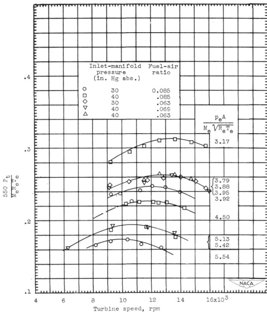
(b) Engine speed, 2400 rpm. Figure 4. - Continued. Variation of blowdown-turbine power with turbine speed.
