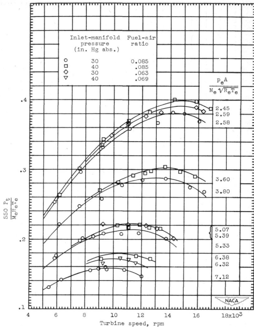
Figure 4. - Variation of blowdown-turbine power with turbine speed.
